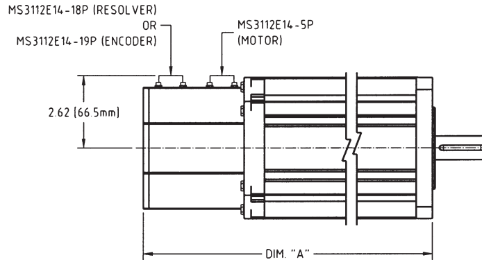
MS CONNECTORS
