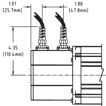
LIQUID TIGHT STRAIN RELIEF WITH FLYING LEADS
