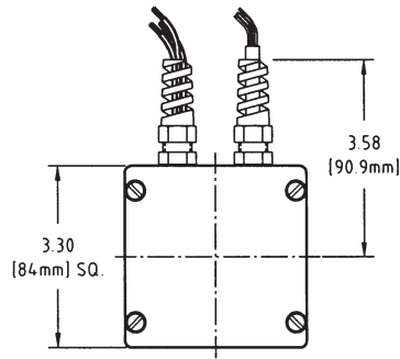
LIQUID TIGHT STRAIN RELIEF WITH FLYING LEADS
