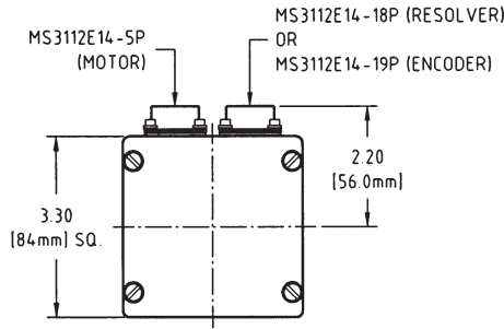
OPTIONAL MS CONNECTOR CONFIGURATION
